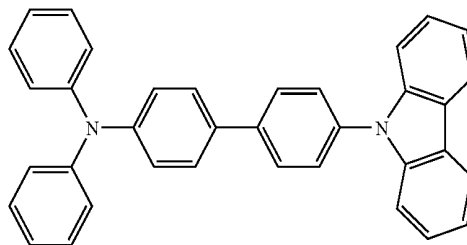
Compound 4-A
