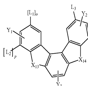
[Chem 14]
