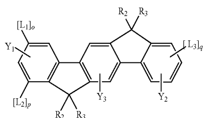
[Chem 2]
