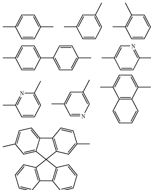
[Chem 114]
