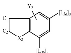
[Chem 7]
