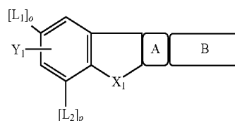
[Chem 4]
