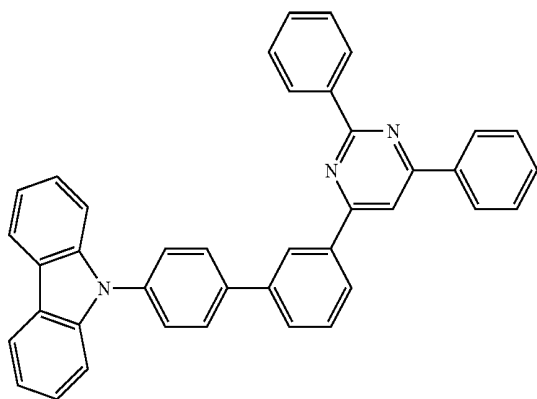
Compound 3-B
