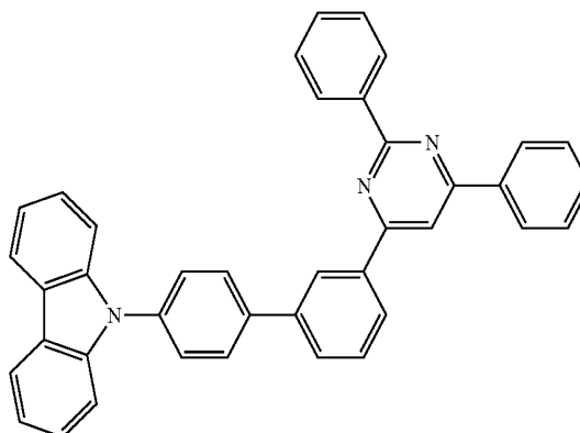
Compound 4-B
