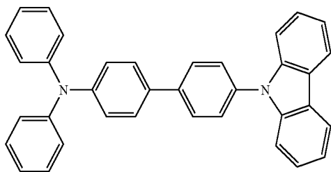
Compound 3-A
