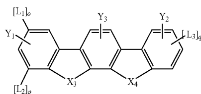
[Chem 8]
