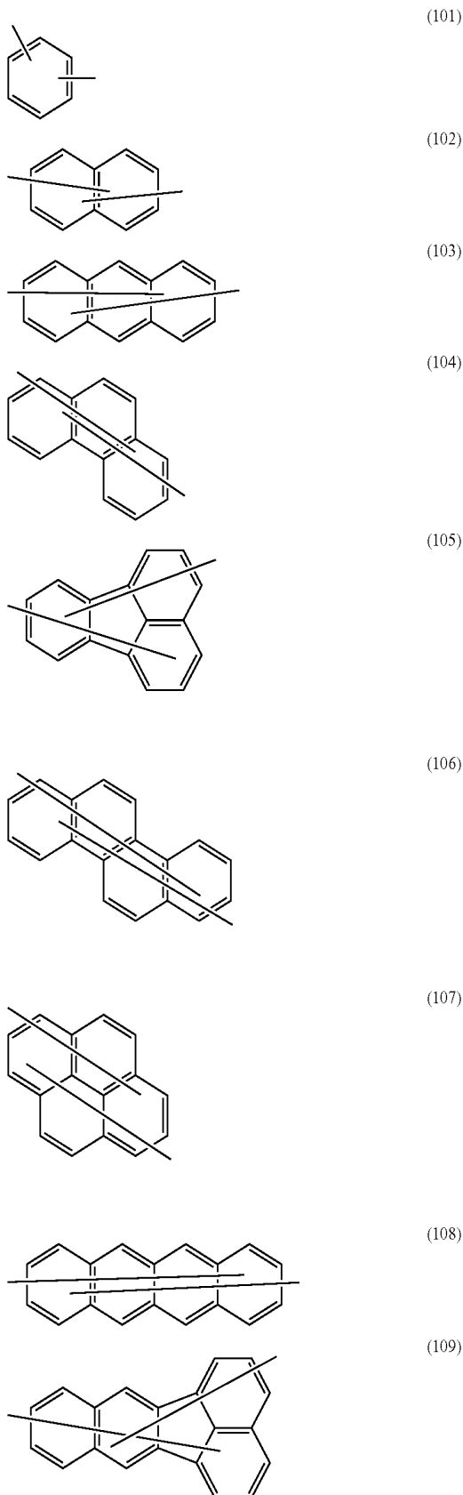
[Chem 115]
